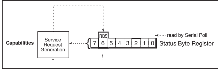
Figure 3 488.1 Status Byte
