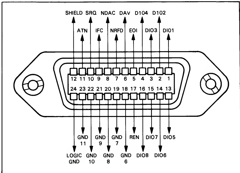
Figure 3-10. The GPIB connector showing pin designations
