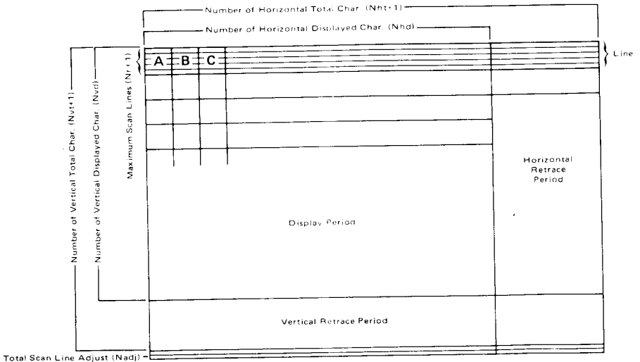
FIGURE 9 - ILLUSTRATION OF THE CRT SCREEN FORMAT
