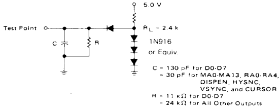
FIGURE 6 – BUS TIMING TEST LOAD
