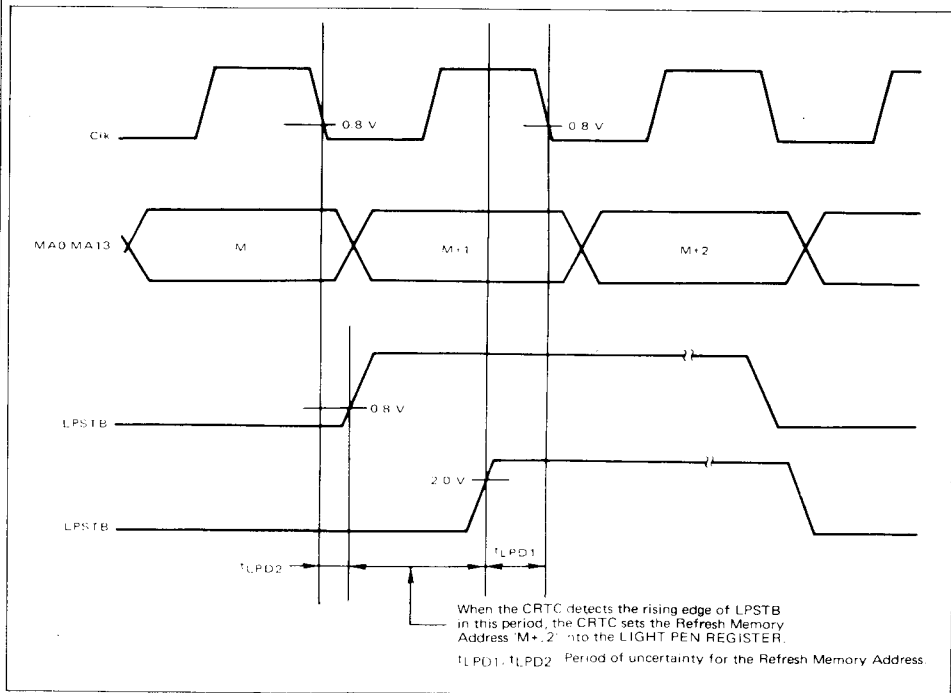
FIGURE 4 - RELATION BETWEEN LPSTB AND REFRESH MEMORY ADDRESS
