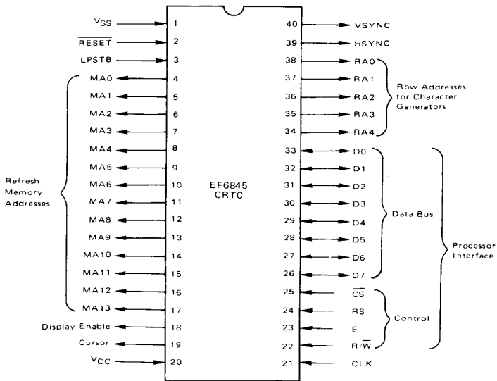
FIGURE 7 – PIN ASSIGNMENT
