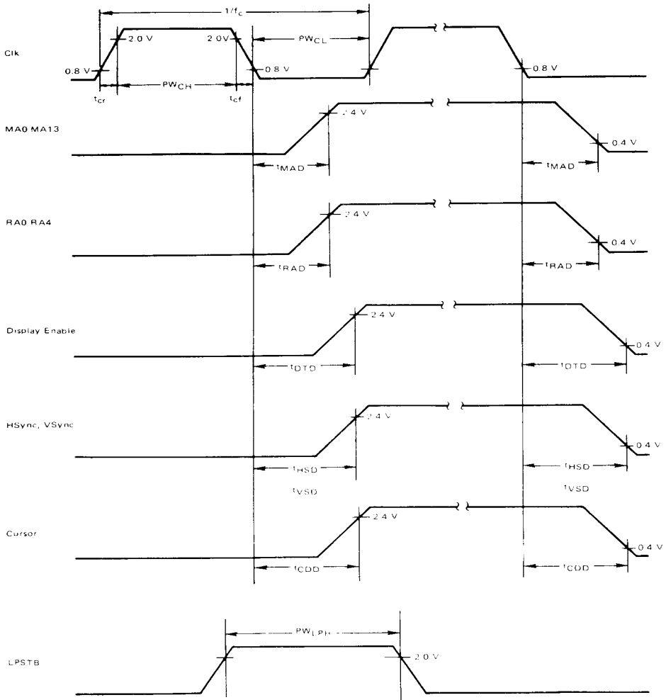
FIGURE 3 - CRTC TIMING CHART
