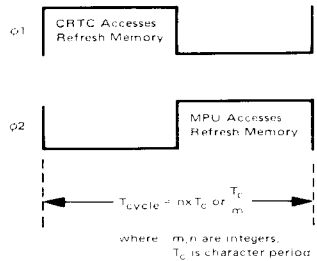
FIGURE 2 - TRANSPARENT REFRESH MEMORY CONFIGURATION TIMING USING 6800 MPU FAMILY
