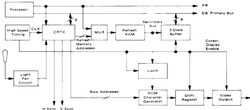
FIGURE 1 - TYPICAL CRT CONTROLLER APPLICATION
