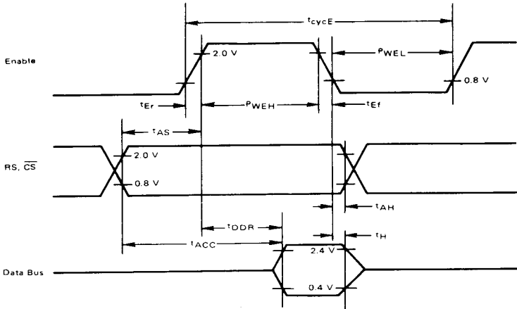
FIGURE 5 - BUS TIMING CHART
