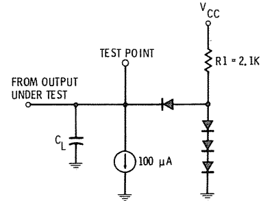
Fig. A-2. Load circuit for output.
