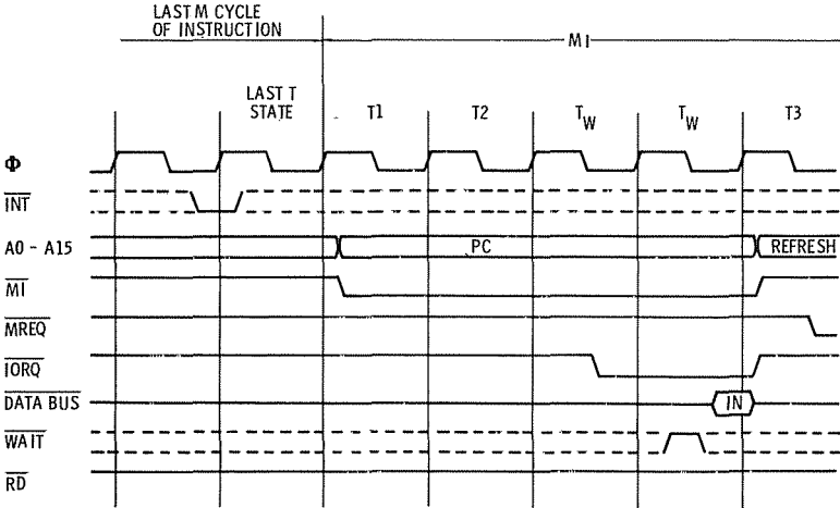
Fig. 3-9. Interrupt Request/Acknowledge cycle.
