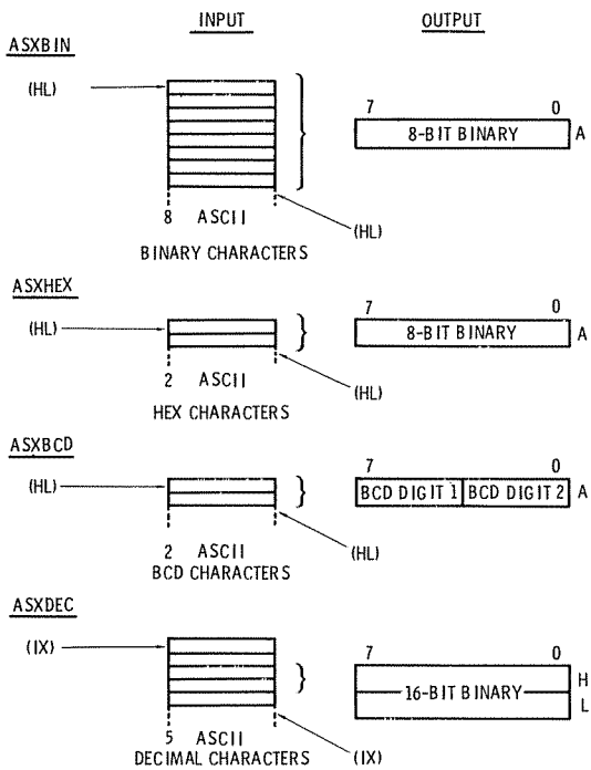
Fig. 16-1. ASCII to base X conversions.
