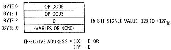
Fig. 4-17. Indexed addressing.
