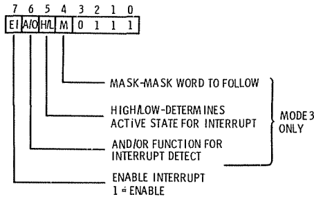
Fig. 8-11. PIO interrupt control word.
