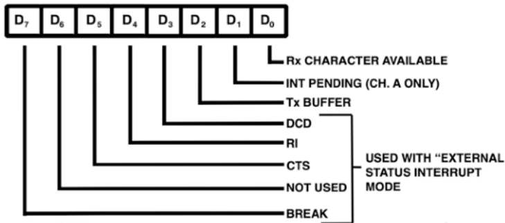
READ REGISTER 0
