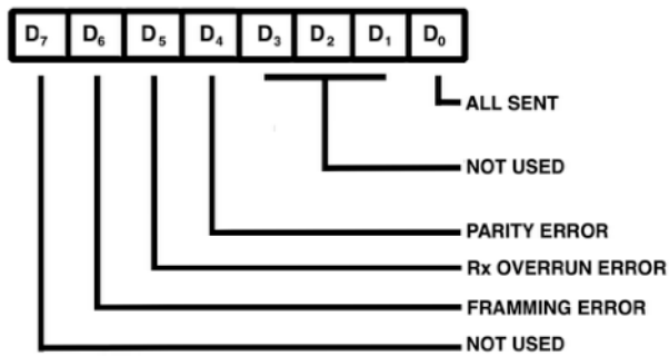
READ REGISTER 1*
