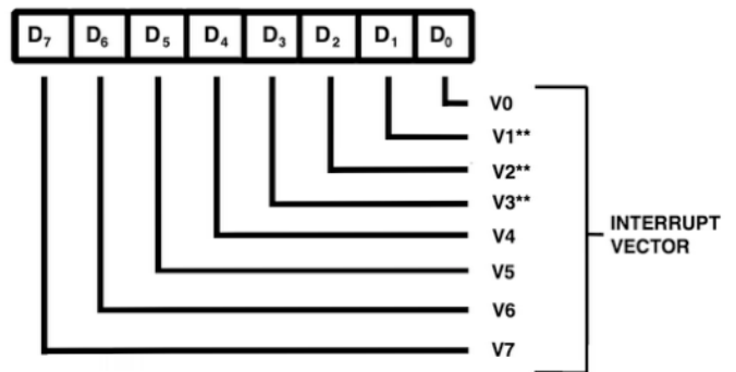
READ REGISTER 2
